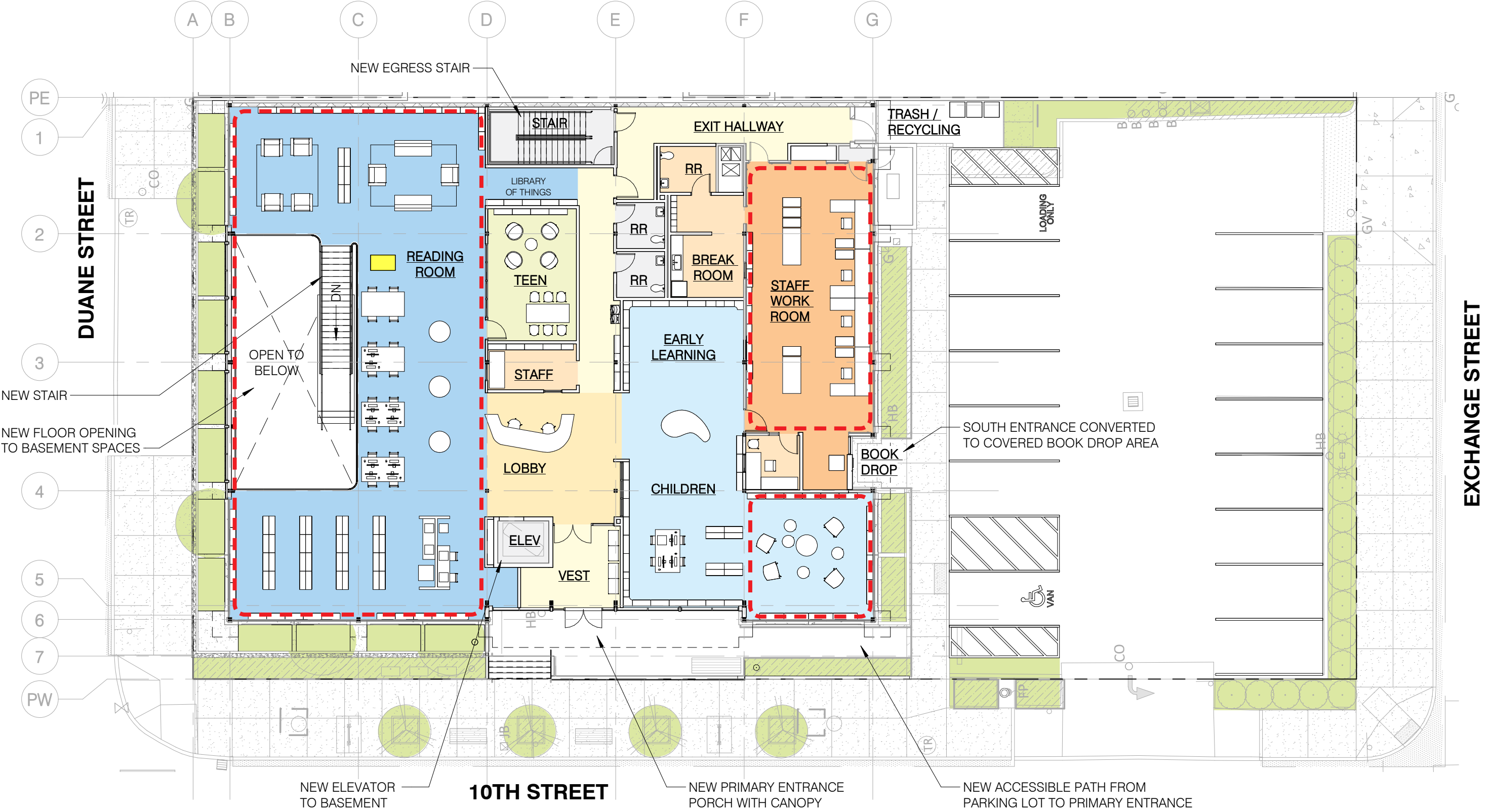
LEVEL 1 FLOOR PLAN - PROPOSED
